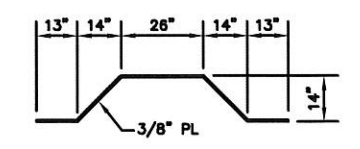
TYPICAL CORRUGATION PROFILE PROFILE TYPICAL FOR LONGITUDINAL & TRANSVERSE BULKHEADS
