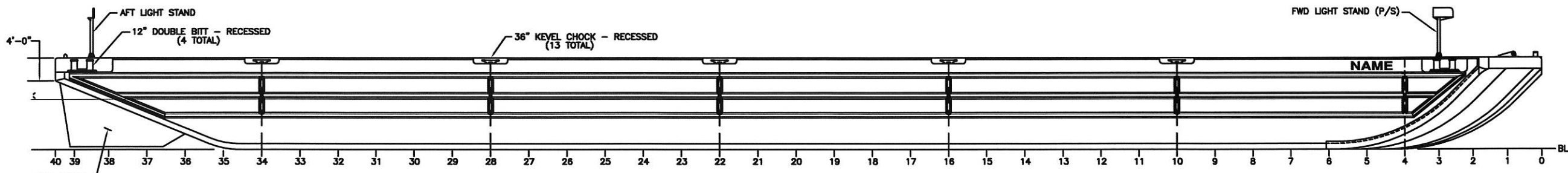
OUTBOARD PROFILE
