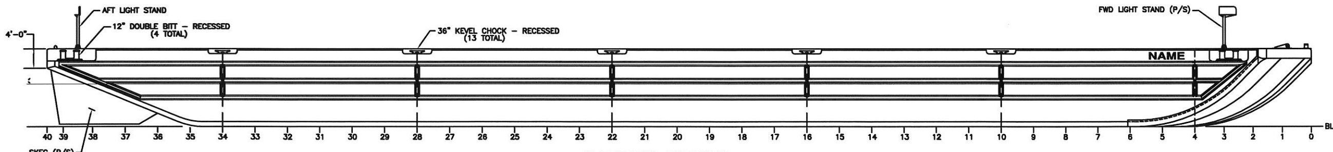
OUTBOARD PROFILE
