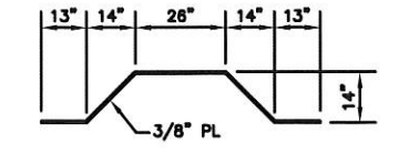
TYPICAL CORRUGATION PROFILE PROFILE TYPICAL FOR LONGITUDINAL & TRANSVERSE BULKHEADS
